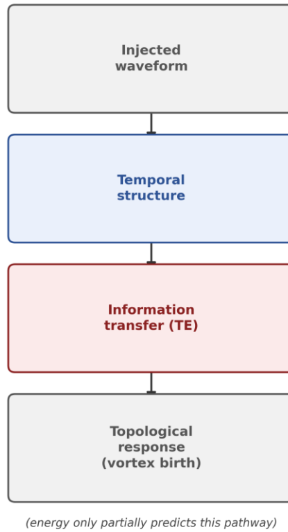
Figure 8. Schematic summary of the pathway established in Section 3. Energy sets a floor on the lattice's response but only partially predicts information transfer or the resulting topological response; temporal structure is the additional variable required to account for both.
